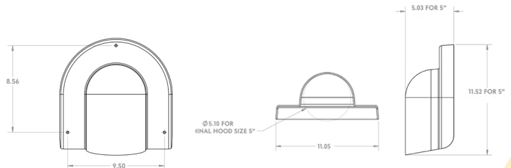
Flash 5™ CAD Drawings with Dimensions
